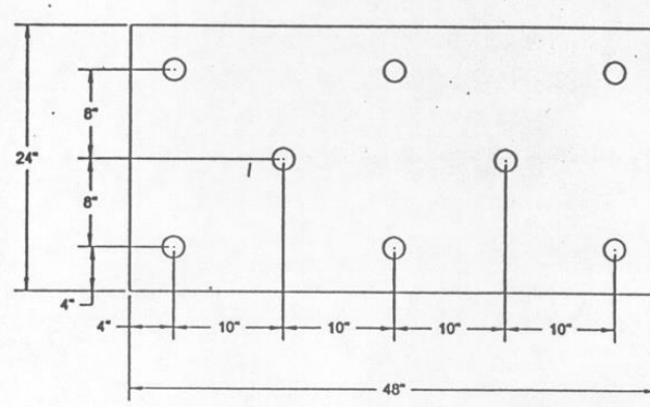
Pattern "D" - For use with structural substrates such as: wood sheathing, concrete, masonry, metal siding
