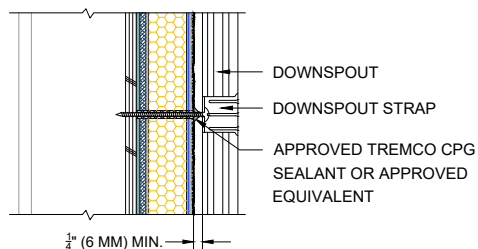
DOWNSPOUT ATTACHMENT
