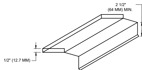
SILL PAN FLASHING DETAIL
