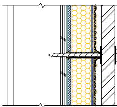
SHUTTER ATTACHMENT
